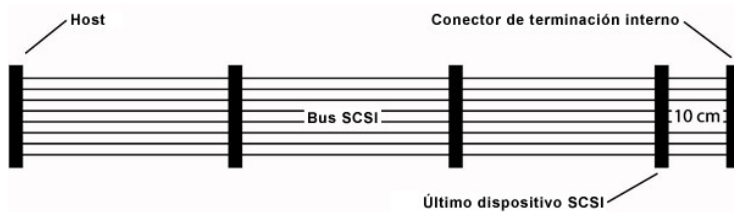
Figura 2: cable SCSI
